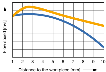
Flow speed depending on the distance to the workpiece
